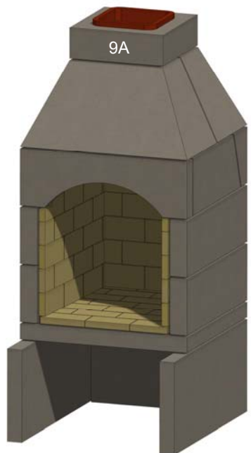
Figure 22. Chimney Flue
