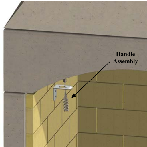
Figure 30. Bracket and Handle Assembly
