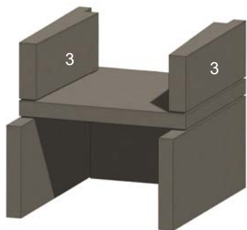
Figure 11. Lower Sidewalls
