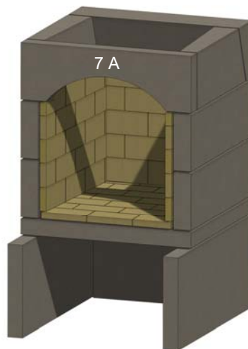
Figure 20. Front Lintel
