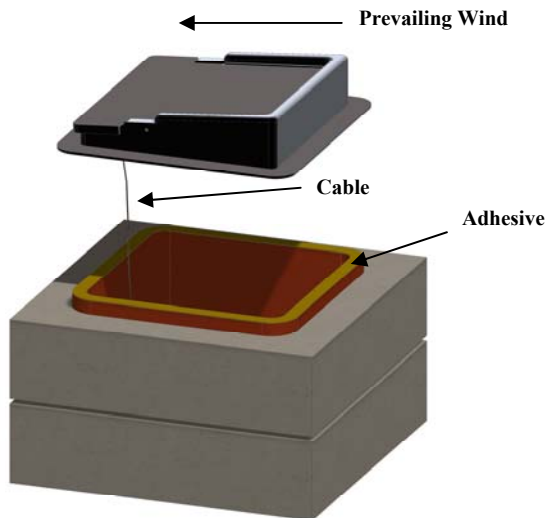
Figure 28. Install Top-Mount Damper
