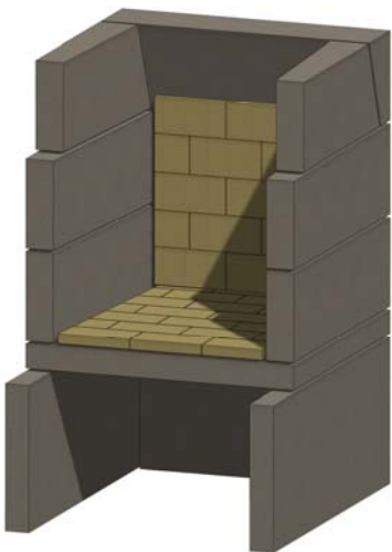
Figure 18. Back Wall Firebrick
