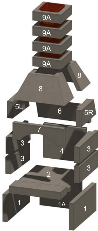
Figure 2. Fireplace Components
