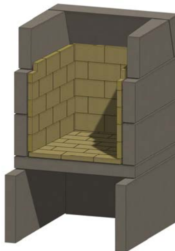
Figure 19. Sidewall Firebrick
