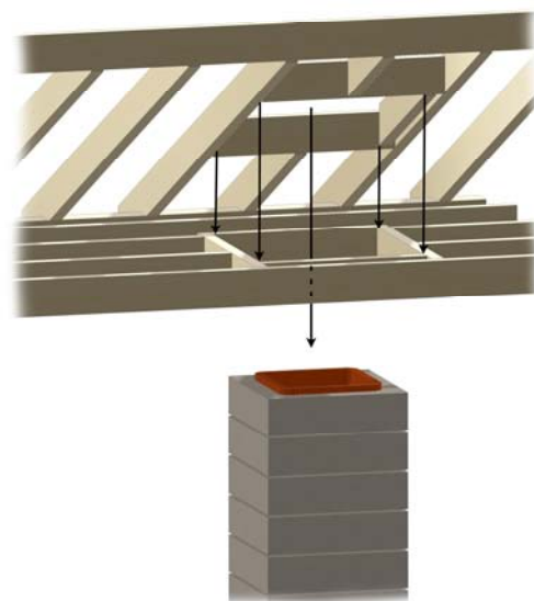
Figure 25. Roof Penetration
