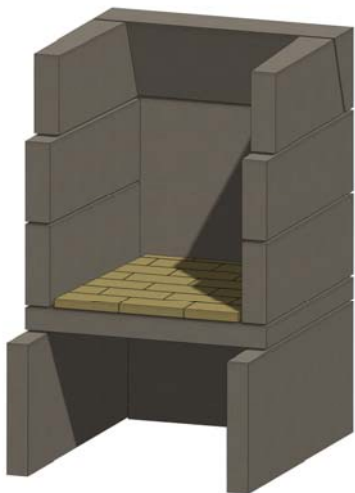
Figure 17. Floor Firebrick
