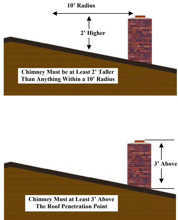
Figure 27. Chimney Height
