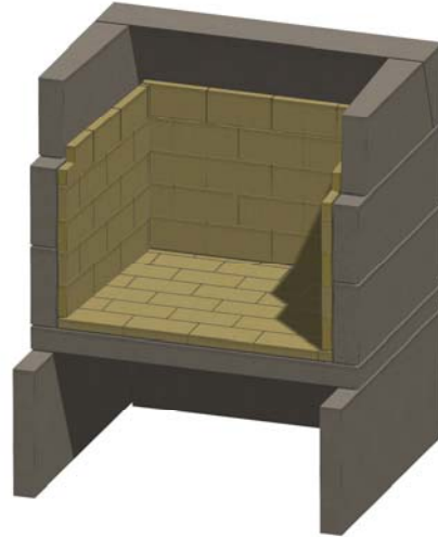
Figure 19. Sidewall Firebrick
